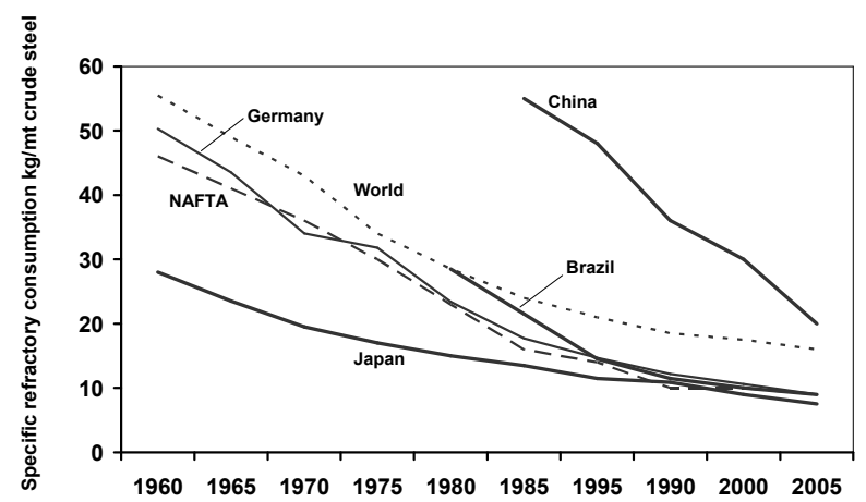
Fig. 5: Steel industry specific refractory consumption trend [8-12]
