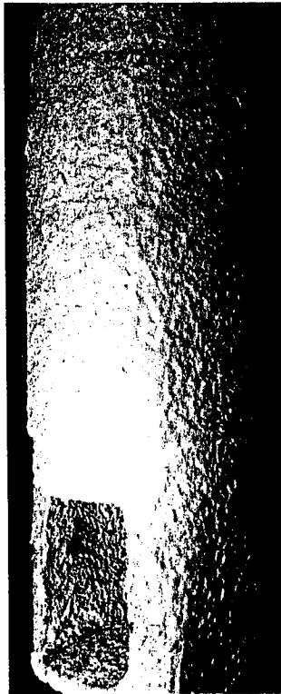
Fig. 3 Submerged nozzle with sprayed on microporous insulation
