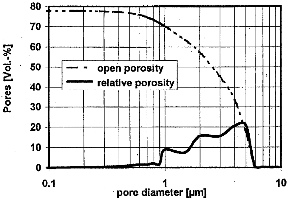
Fig 2: Micro pore size distribution of SLA-92 (Hg-intrusion method) [5]
