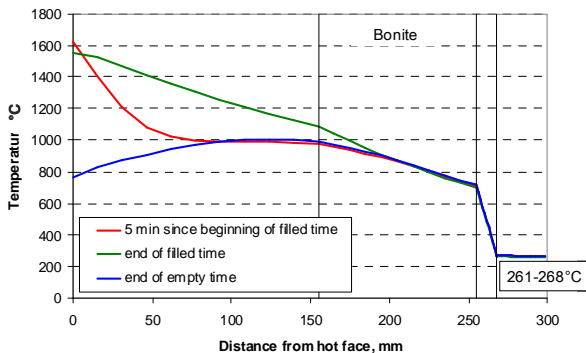
Fig. 6 Temperature distribution in the “new” lining (left) and old/worn lining (right) (155 mm AMC-brick, 100 mm BONITE castable, 13 mm Vermiculite board)
