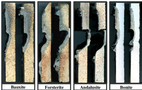
Fig. 3. Samples after slag test; CaO/Al 2 O 3 -ratio 1.08 (Induction furnace, 1600 °C / 2 h; air)
