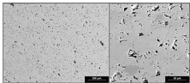
Fig. 1. Microstructure of Bonite (polished section). Hexagonal CA_6 platelets and few pores in between.
