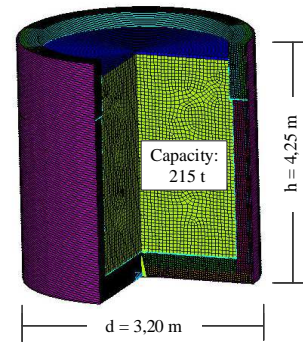
Fig. 4. Transient, two-dimensional, and axis-symmetrical FEM model of a steel ladle.
