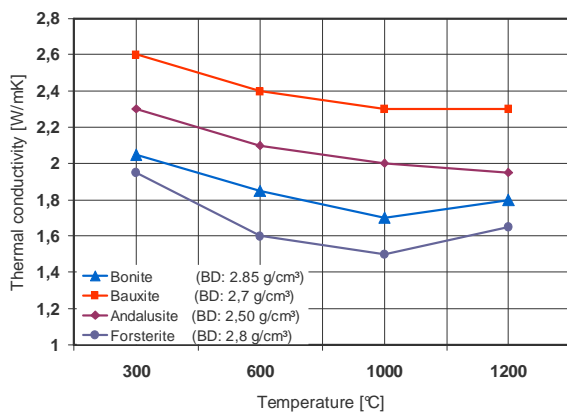
Fig. 2. Thermal conductivity of refractory materials used for steel ladle permanent linings [4].
