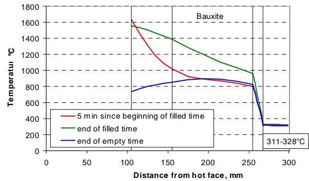
Fig. 5 Temperature distribution in the “new” lining (left) and old/worn lining (right) (155 mm AMC-brick, 100 mm bauxite castable, 13 mm vermiculite board)
