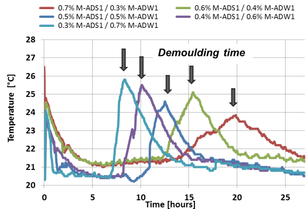
Fig. 1: Dispersing Alumina combinations and their influence on castable setting. Exothermic reaction of a low cement castable with 5% silica fume.
